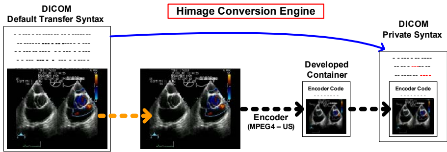
Fig. 1. Conversion of DICOM “default transfer syntax” in “private syntax”
