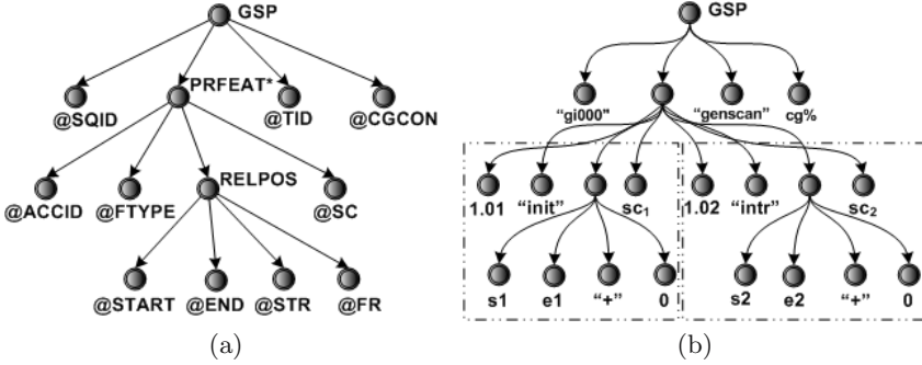
Fig. 2. (a) Hierarchical view of the XIS (* indicates potential repeated elements and @ denotes valued schema elements) and (b) an example well-formed XML document containing sample values
