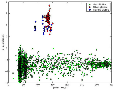
Fig. 4. Z-score plot for sequence classification using \lambda -dec measure based profiles
