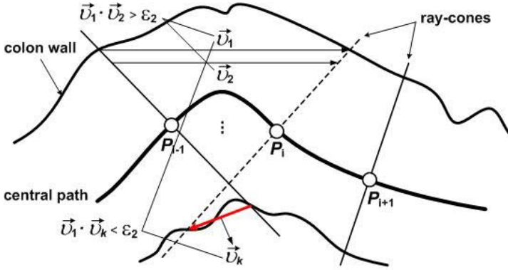
Fig. 7. Illustration of intersection test: Vector \vec{U} is defined as direction vector that has identical index in two consecutive ray-cones
