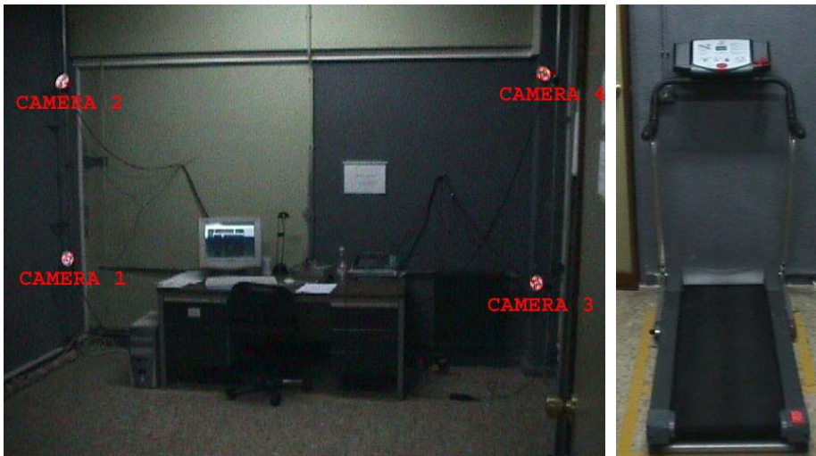
Fig. 1. Stereovision system composed by four cameras, frame-grabber and PC, and the conveyor belt
