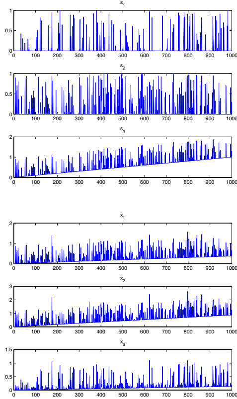
Fig. 3. Top: The original sources \mathbf{s}_i . Note, that \mathbf{s}_3 was obtained from \mathbf{s}_2 by adding a linear function. Bottom: The rows \mathbf{x}_i of the mixture matrix \mathbf{X} as provided to the algorithms
