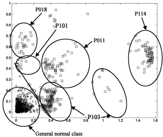
Fig. 7. Clusters of heartbeats representing the normal and the premature ventricular excitations for 5 patients (P011, P018, P101, P103, P114) represented by modified PCA descriptors and the linear SVM classifier
