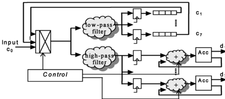
Fig. 4. Wavelet transform module architecture overview
