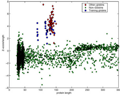
Fig. 2. Z-score plot for sequence classification using probability measure based profiles
