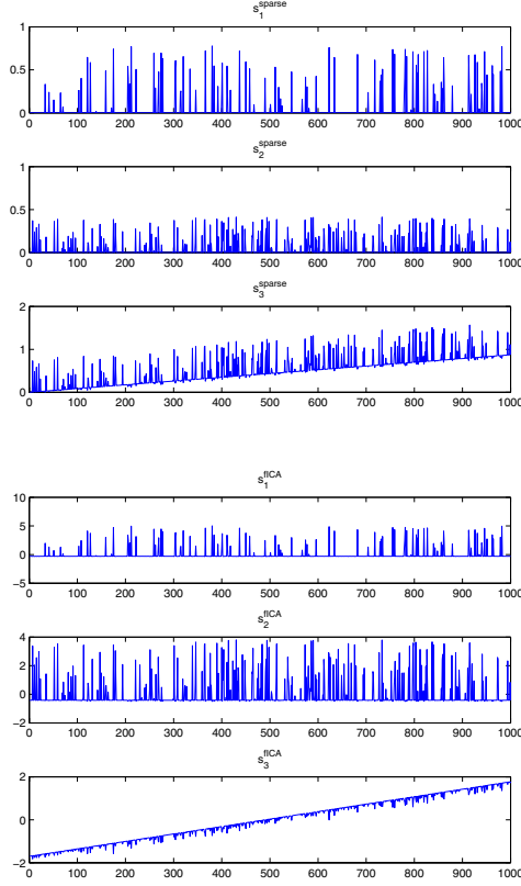
Fig. 4. Top: The estimates s_i^{sparse} of the sources as obtained by the nonnegative sparse BSS algorithm. Bottom: The estimates s_i^{fICA} of the sources as obtained by the fastICA algorithm. Note, that fastICA fails to recover the third source
