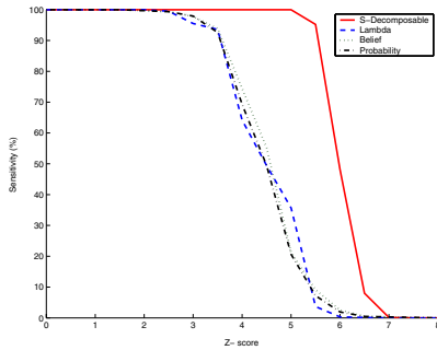
Fig. 8. Sensitivity curve for different measures with respect to Z-score cutoffs
