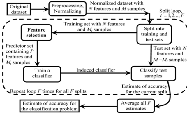
Fig. 1. F -splits procedure
