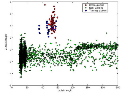
Fig. 5. Z-score plot for sequence classification using belief measure based profiles
