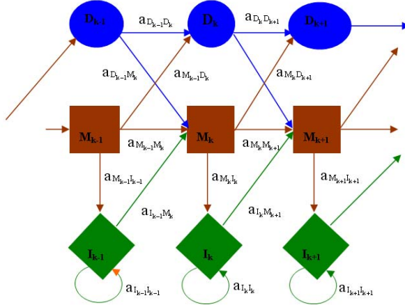
Fig. 1. Plan 7 architecture of Profile HMM used in HMMER 2 [7]. This architecture differs from the original (Plan 9) Krogh/Hausler architecture also used in earlier versions of HMMER by reducing the number of transitions from 9 to 7. It has no D \rightarrow I and I \rightarrow D transitions. The equations for fuzzy profile HMM are formulated based on the plan 9 architecture. The fuzzy model for plan 7 architecture can be easily obtained by setting the transition parameters a_{D_k I_k} and a_{I_{k-1} D_k} to zero in all the equations wherever they appear
