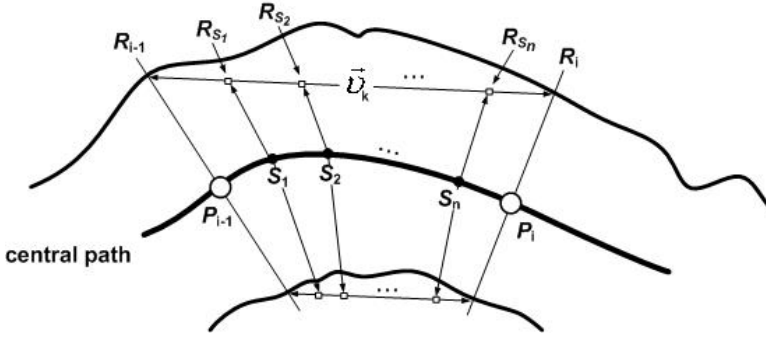
Fig. 8. Example of linear interpolation for direction of rays on sample points using ray-cones on control points. White circles are control points and black ones are sample points
